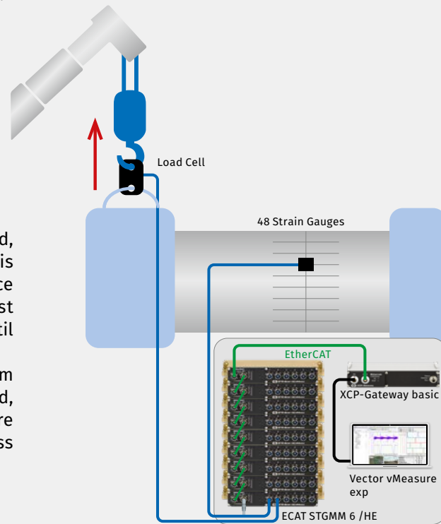
Fig. 4: The measurement modules are transported to the test area with the test specimen. Here, the test specimen is fixed on one side and the desired load is applied by lifting on the other end.
