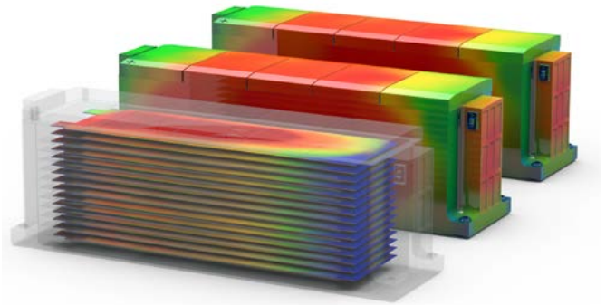
Fig. 4: Precise temperature measurements on the pouch cells and battery blocks are necessary to trace the spread of temperatures in the battery housing.
