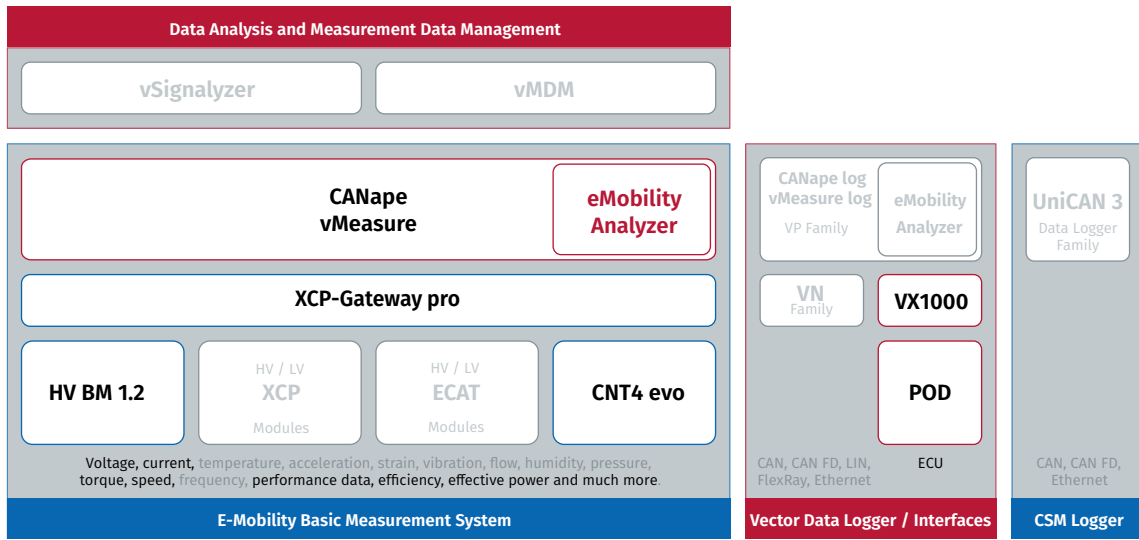
Fig. 4: The efficiency measurement of a HV powertrain in the systematics of the Vector CSM E-Mobility Measurement System
