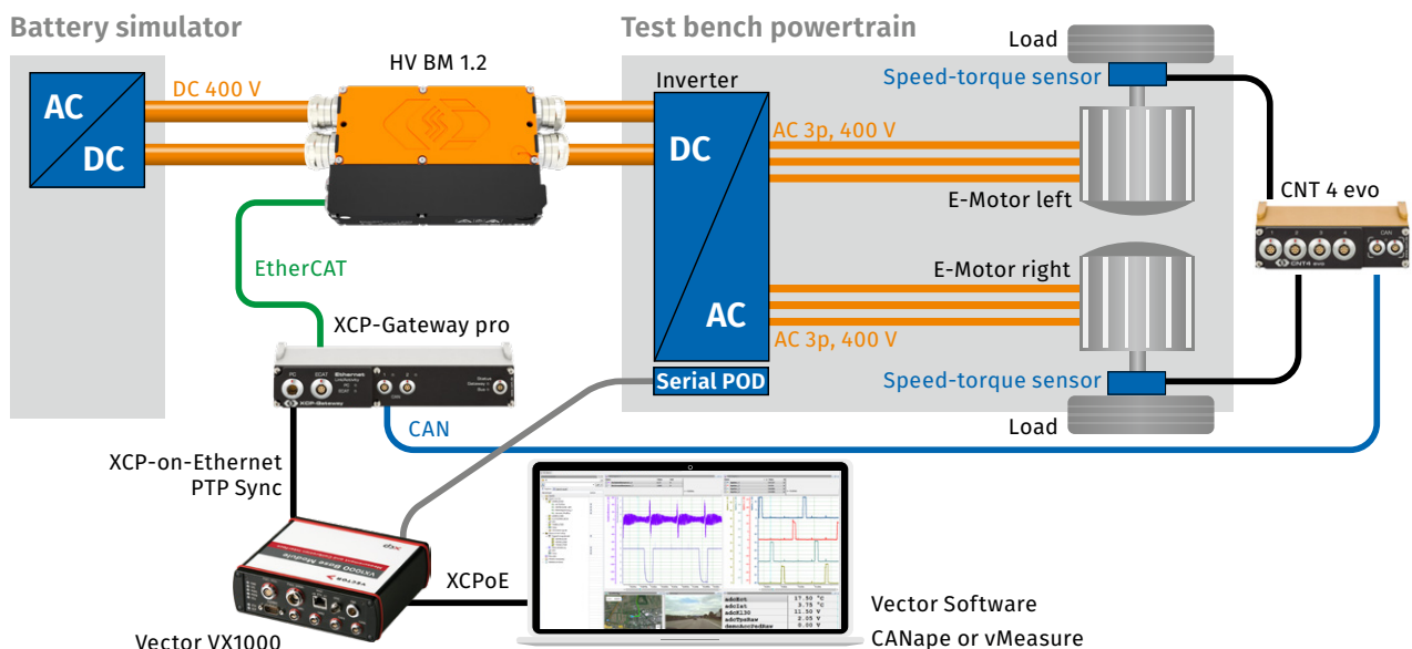
Fig. 1: Vector CSM E-Mobility Measurement System for efficiency analysis of a powertrain. The eMobilityAnalyzer for power analysis is an integral part of Vector CANape and vMeasure software.
