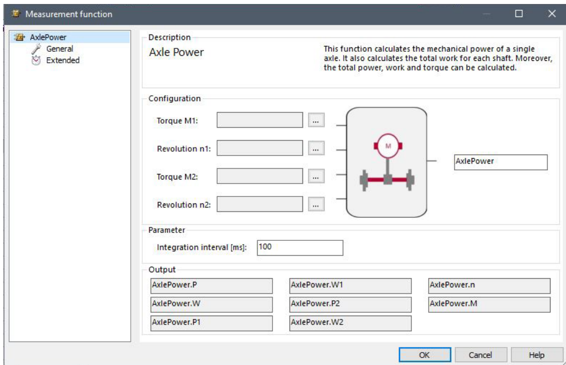
Fig. 3: The Axle Power function calculates the mechanical performance and total power from the signals of the speed torque sensors on the each of the two axles
