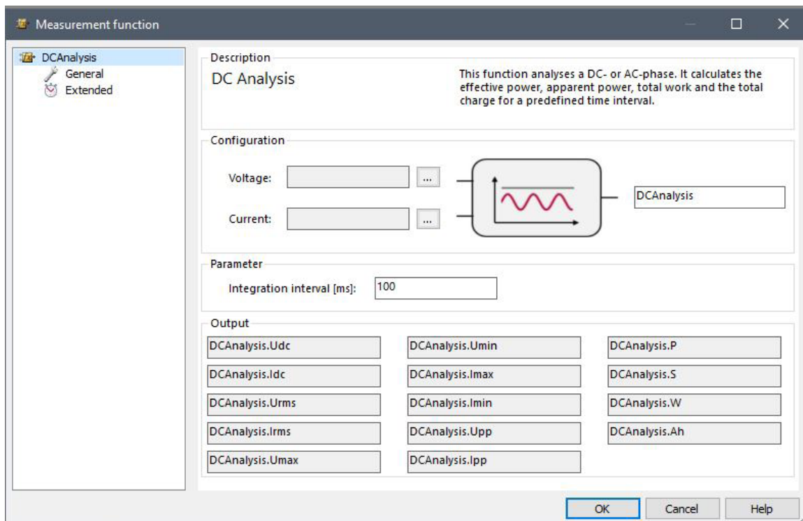
Fig. 2: The DC Analysis function for power analysis on a DC line. The input variables are the sampling values of voltage and current from the HV BM 1.2. The effective power, apparent power, total work, and total load are calculated from a predetermined equation.
