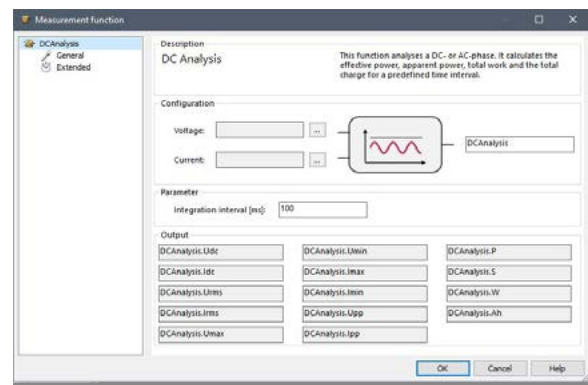
Fig. 2: The DC Analysis function for power analysis on a DC line. The input variables are the sampling values of voltage and current from the HV BM 1.2. The effective power, apparent power, total work, and total load are calculated from a predetermined equation.
