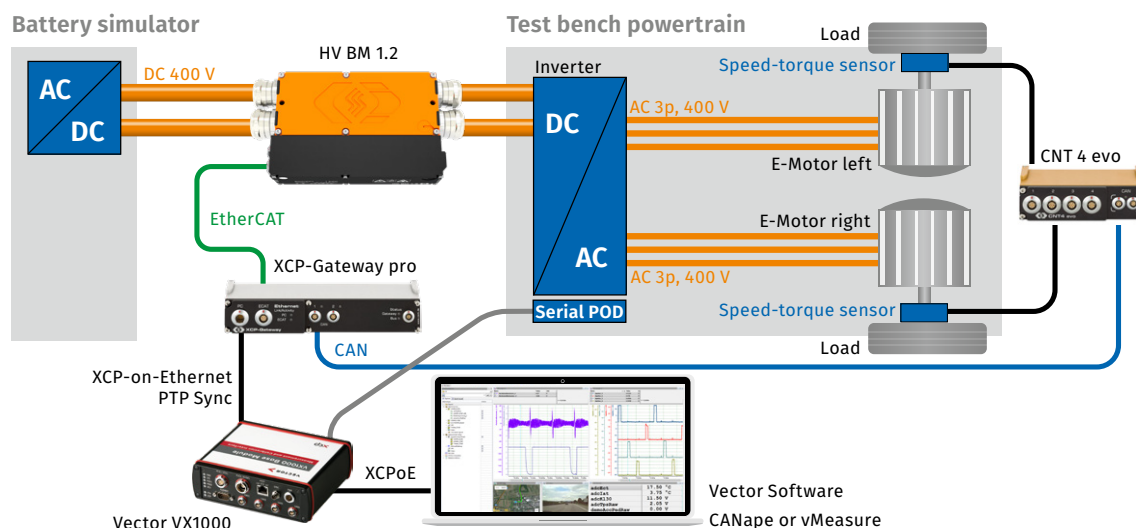
Fig. 1: Vector CSM E-Mobility Measurement System for efficiency analysis of a powertrain. The eMobilityAnalyzer for power analysis is an integral part of Vector CANape and vMeasure software.
