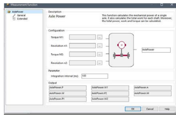
Fig. 3: The Axle Power function calculates the mechanical performance and total power from the signals of the speed torque sensors on the each of the two axes
