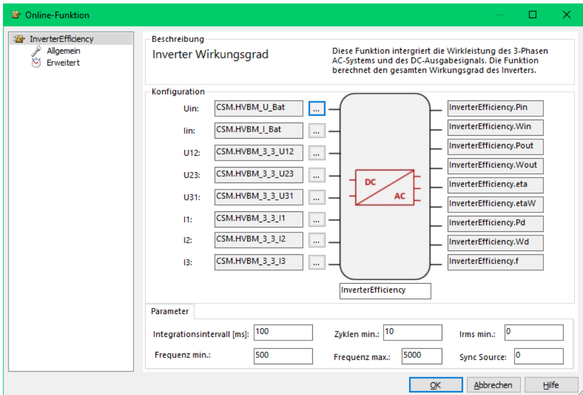
Fig. 4: Efficiency analysis with the eMobilityAnalyzer
