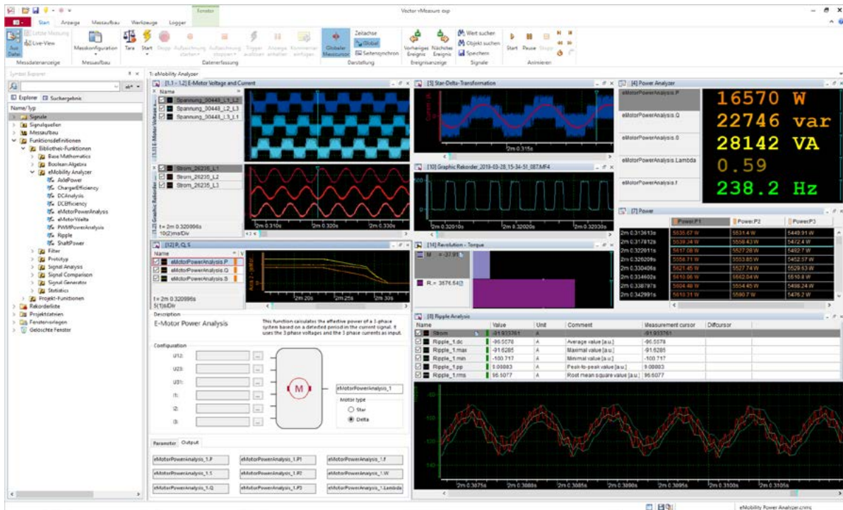
Fig. 3: Vector software vMeasure exp with opened function library eMobilityAnalyzer and power analysis.
