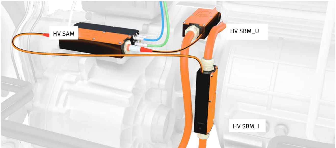
Fig. 1-1: Modular mounting of the measurement technology components
