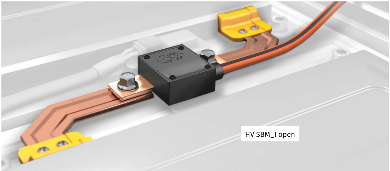
Fig. 1-2: Integration of an HV SBM_I open into a busbar
